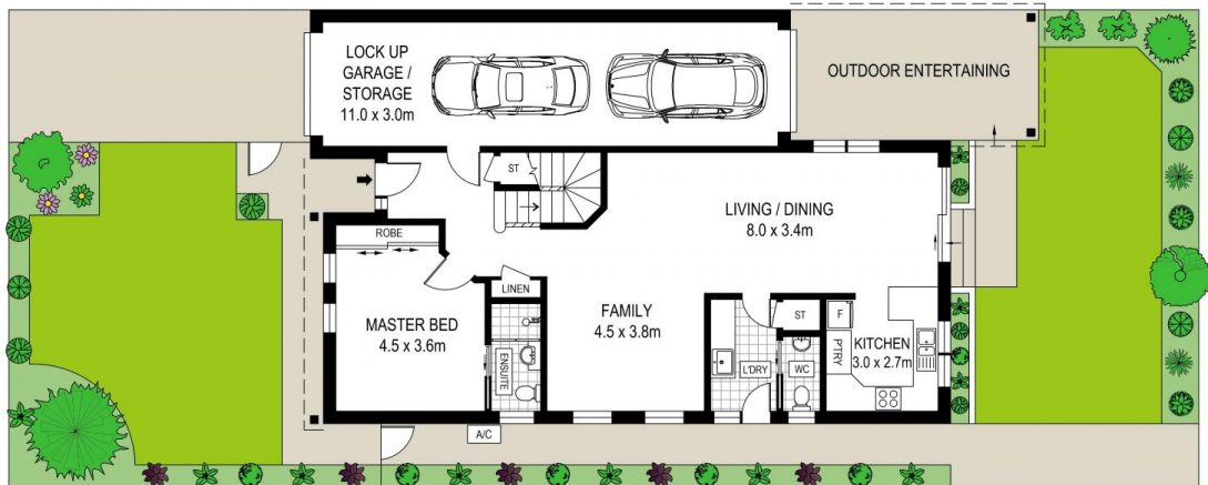
GROUND FLOOR
