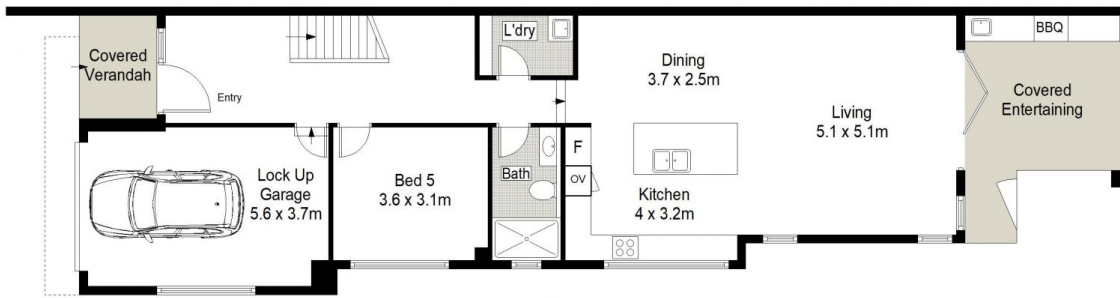
GROUND FLOOR
