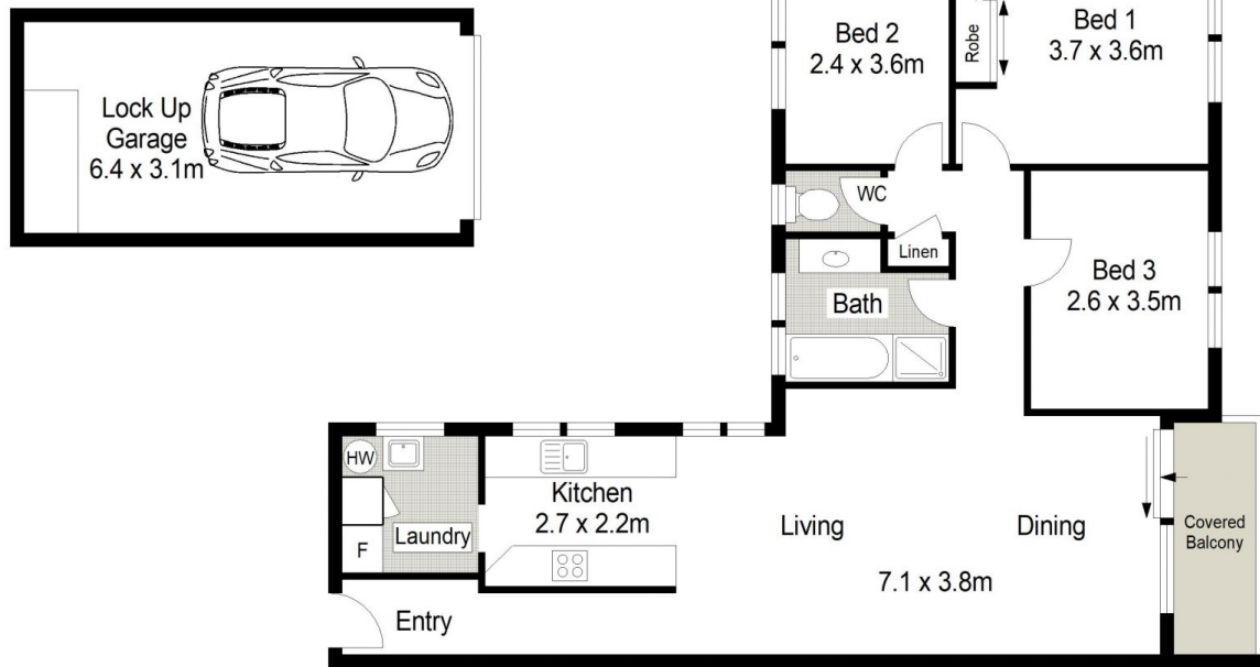
TOP FLOOR
