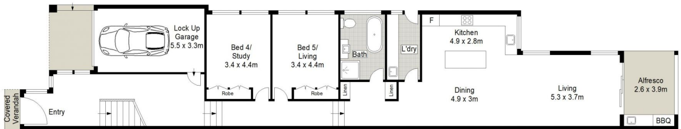
GROUND FLOOR
