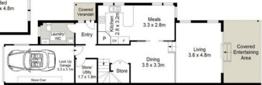
GROUND FLOOR
